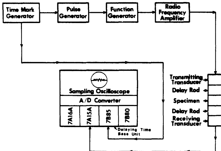
Fig. 1. A schematic of the apparatus.
