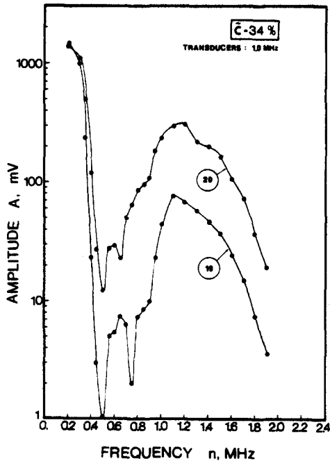
Fig. 5. (a) The minimum amplitude occurs at 0.466 MHz for both specimens. Transducers: 0.5 MHz. (b) When 1.0-MHz transducers are used (instead of 0.5 MHz), the minimum shifts to 0.5 MHz.
